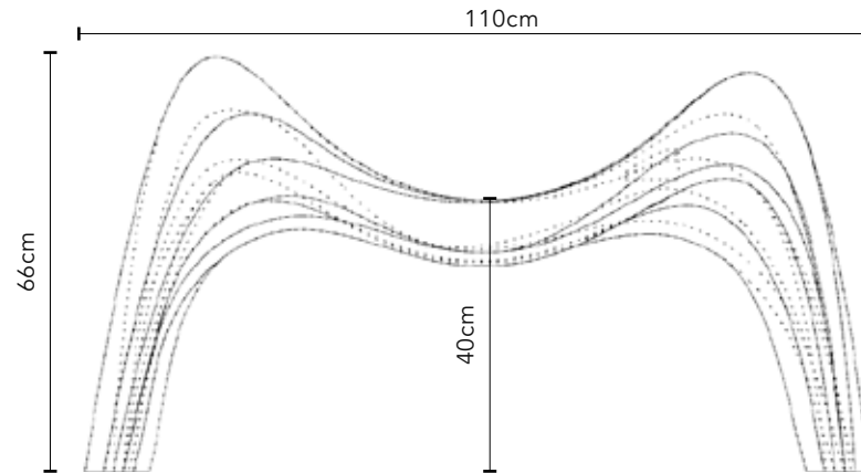
Elevation Large
