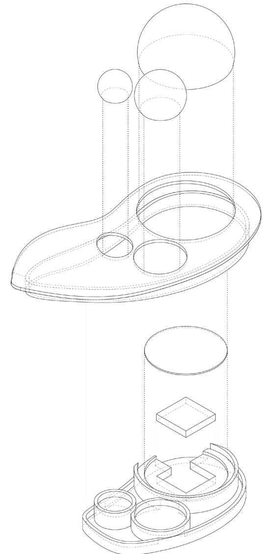
Assembly Drawing
